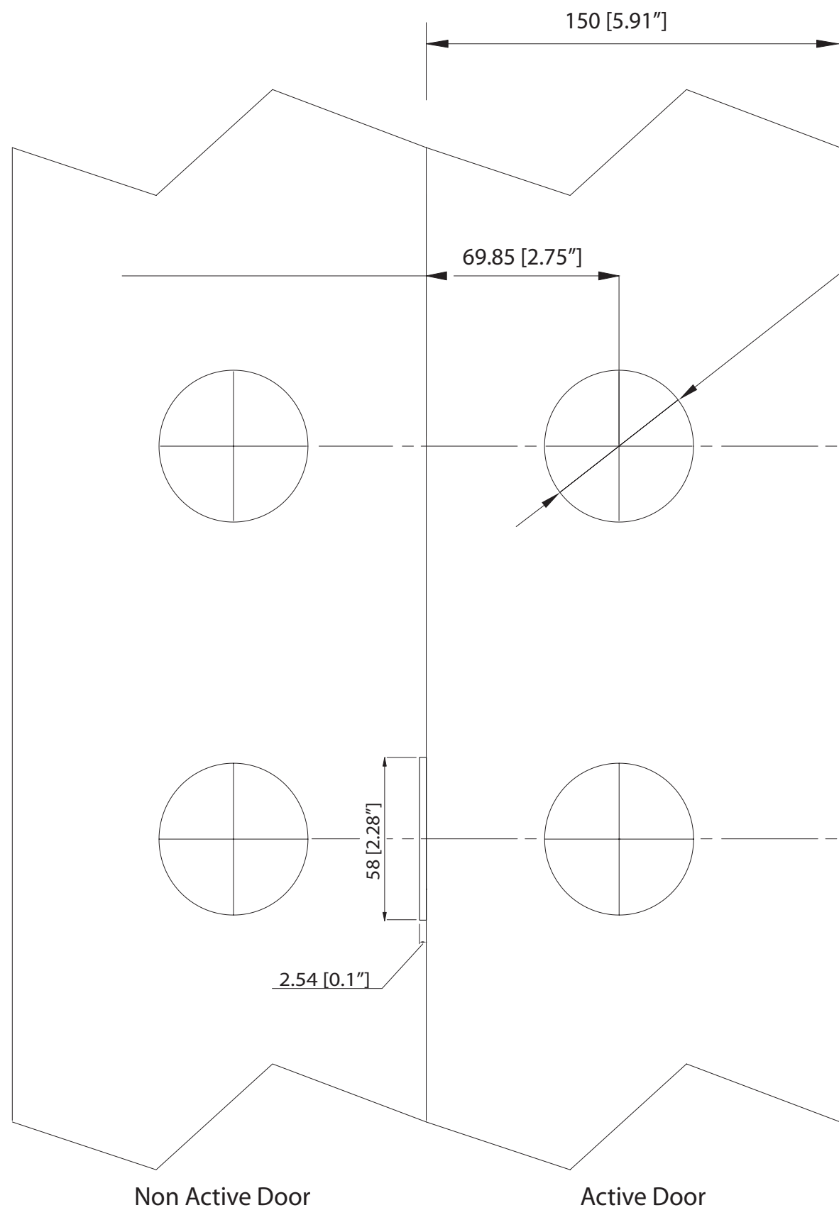
Door Face Borings VIEW FROM INSIDE, BOTH DOORS CLOSED
