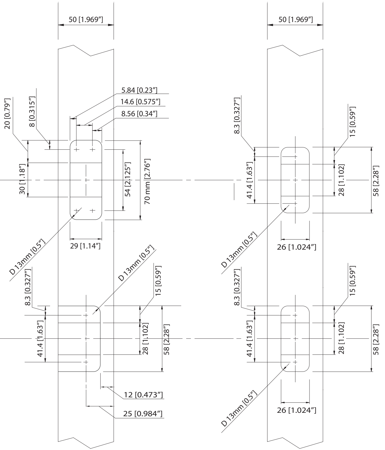
Non Active Door Striker Plate Cutouts
